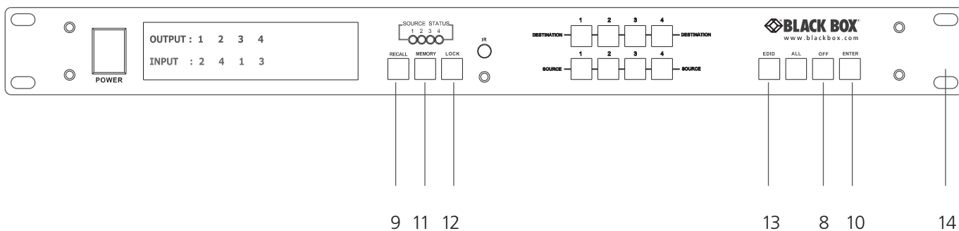
Figure 2-2. Front-panel diagram #2.
