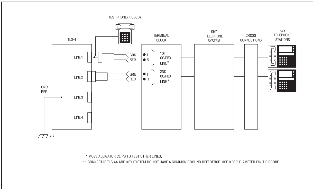
Figure 5 Key System Test Connections
