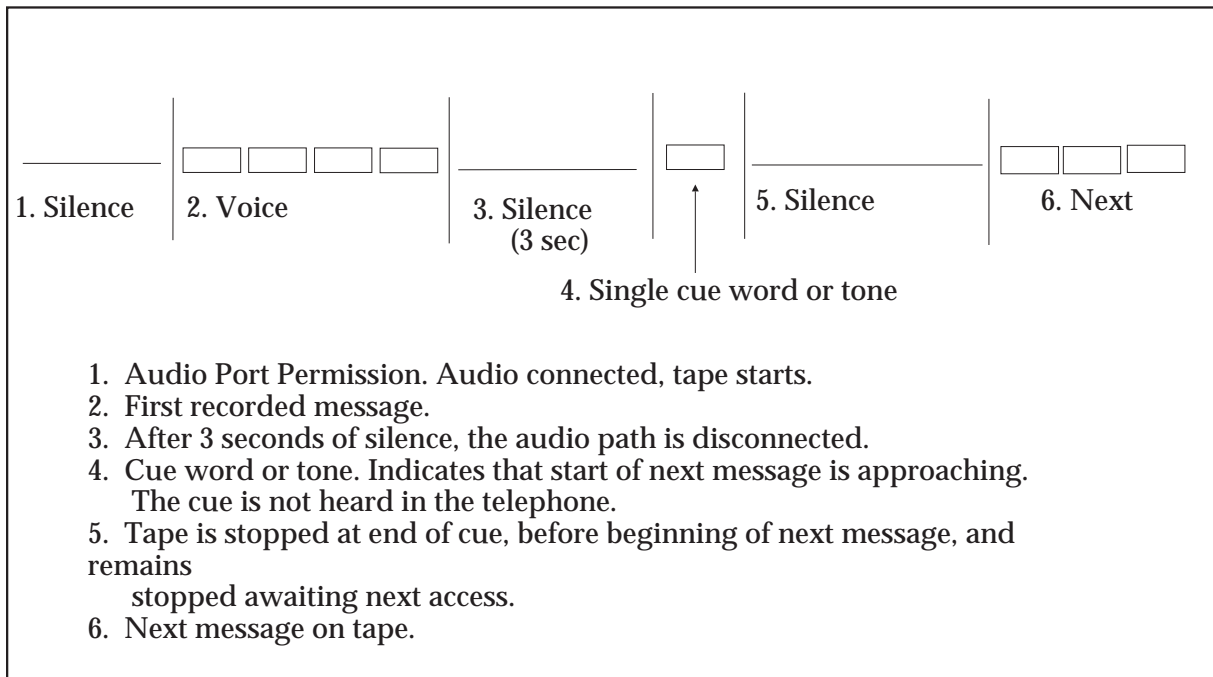
Figure 3 End of Message Tape Sequence
