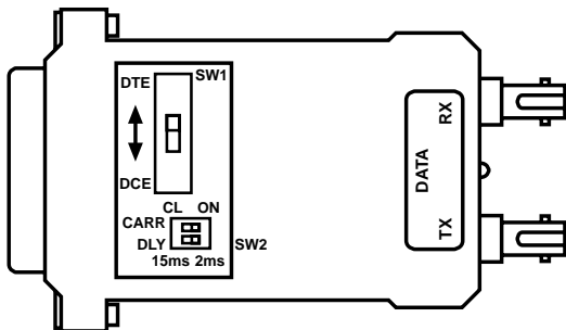
Figure 3-1. Strapping diagram.
