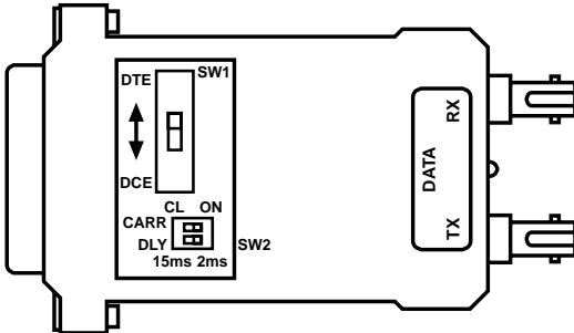
Figure 3-1. Strapping diagram.
