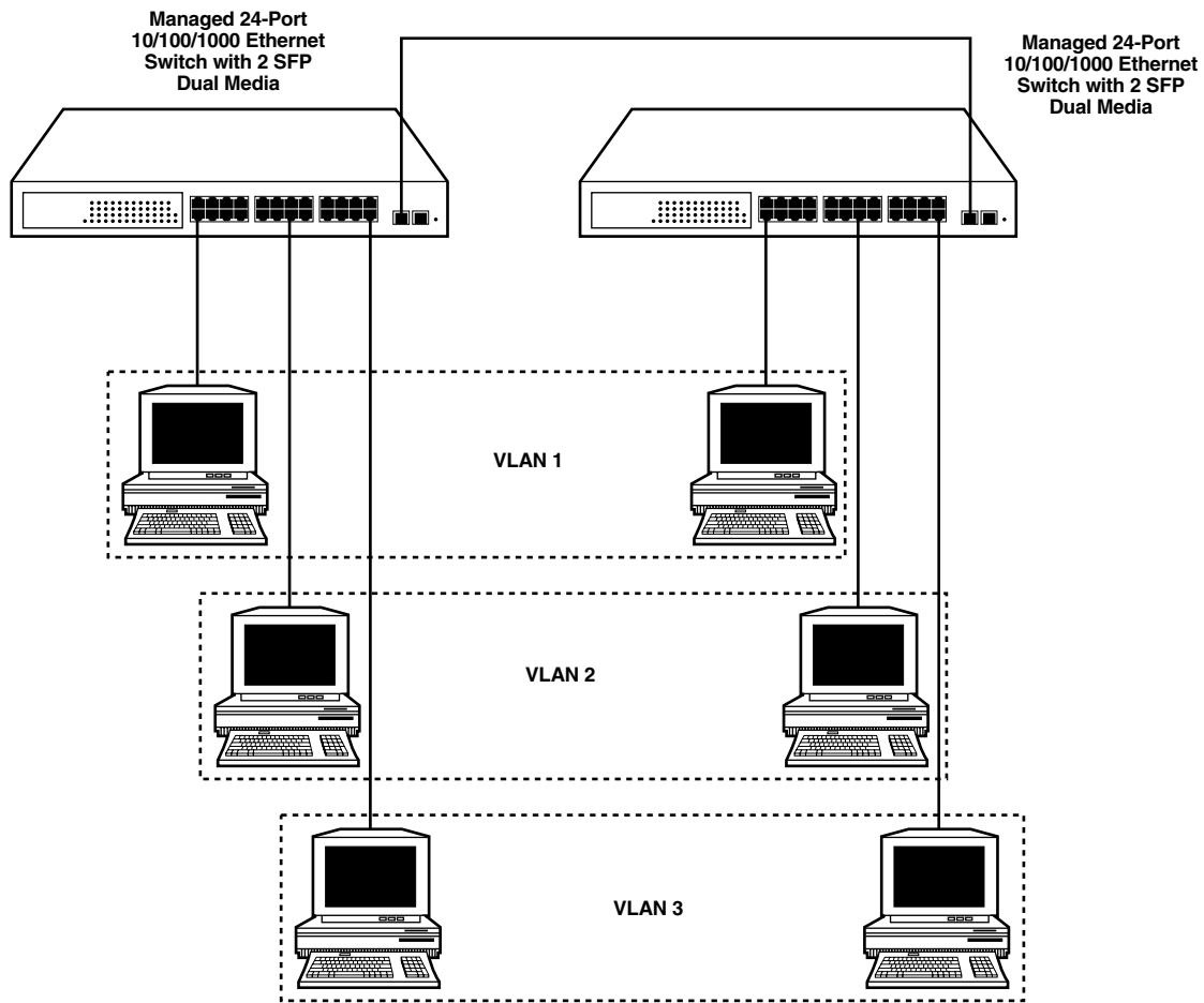
Figure 3-4. Attribute-based VLAN diagram.
