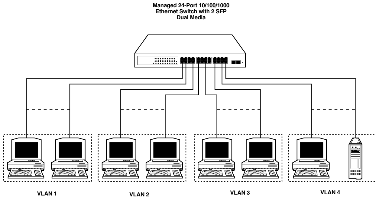
Figure 3-3. Port-based VLAN.
