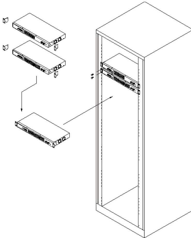
Figure 3-2. Chassis installation.
