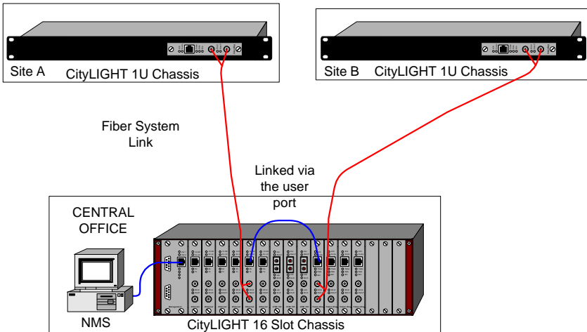
Figure 3 - Linking Two Sites Managed from a Central Office
