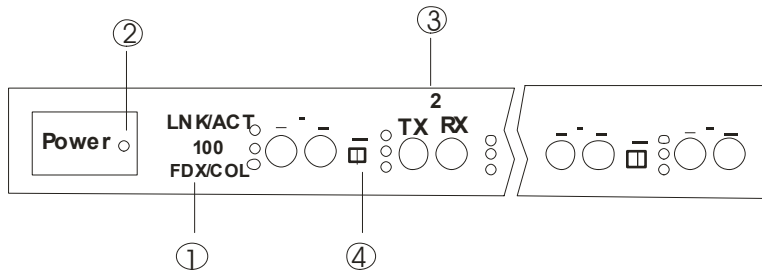
Figure 2: Port status display LEDs of LB9009A-FO.
