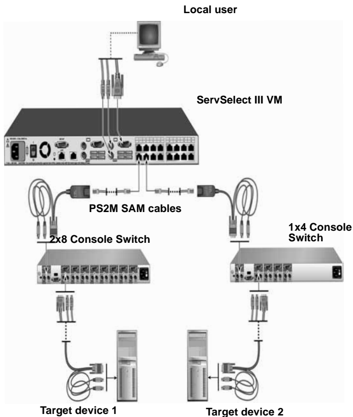
Figure 3-3. Appliance configuration with an earlier-model appliance
