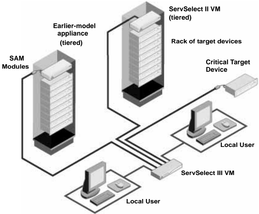
Figure 2-2. Example ServSelect III VM appliance configuration
