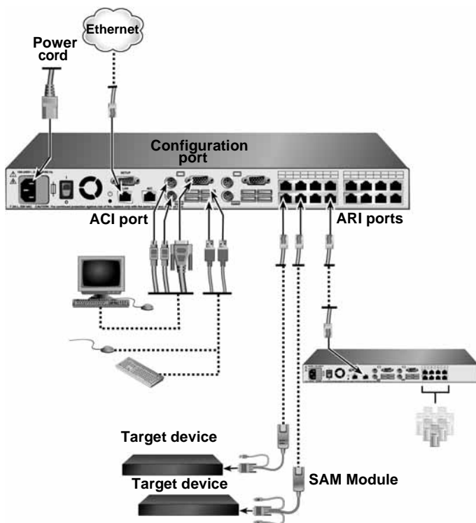
Figure 3-1. ServSelect III VM configuration example
