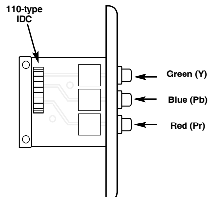
Figure 2-1. Component Video UTP Wallmount Module.
