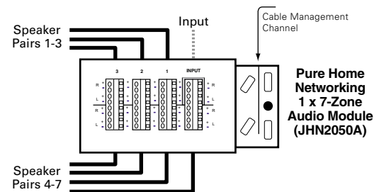
Figure 3-1. Typical setup.
