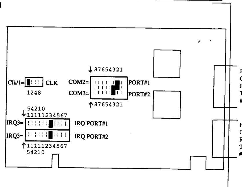
Figure 2-2. AT Velocity RS232 Card Layout.
