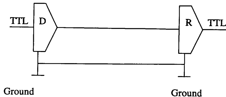
Figure 2-1. RS232 Point To Point Connection.
