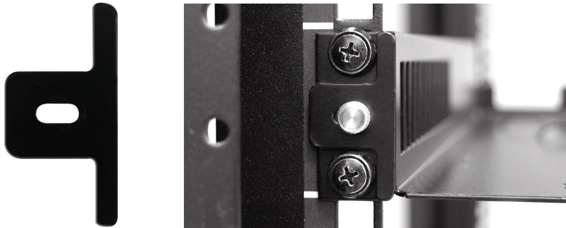
FIGURE 2-4. INSTALL THE LOCKING BRACKET
