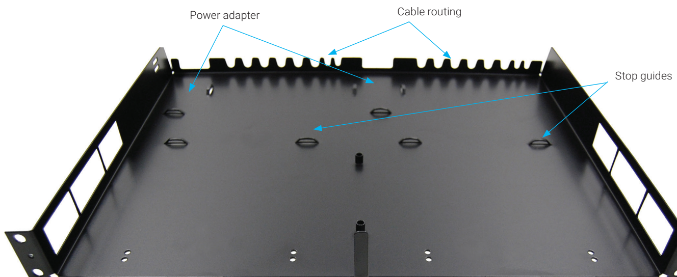
FIGURE 1-1. INSIDE OF THE RACKMOUNT TRAY
