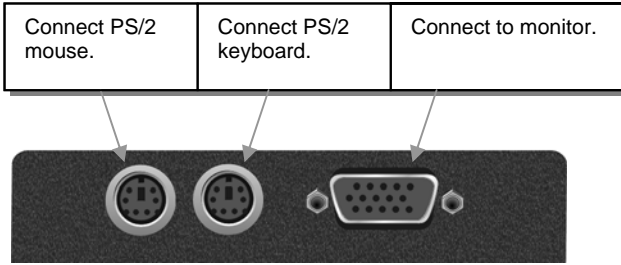
Standard Remote Unit/Hub Port – rear view (ACUMREM, ACU3001A, ACU3009A, ACU1006MRA)
