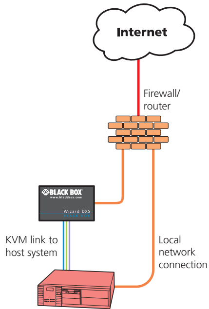
Figure E-1. Wizard DXS - Digital situated behind the firewall
