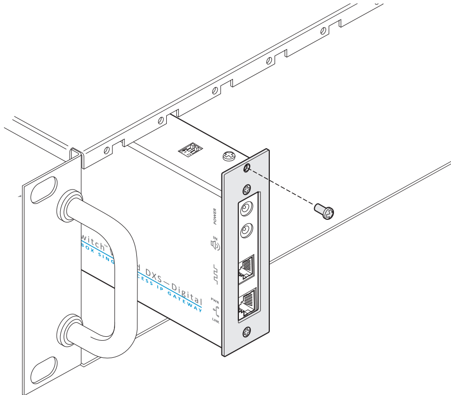
Figure 3-2. Fixing the module into the rack
