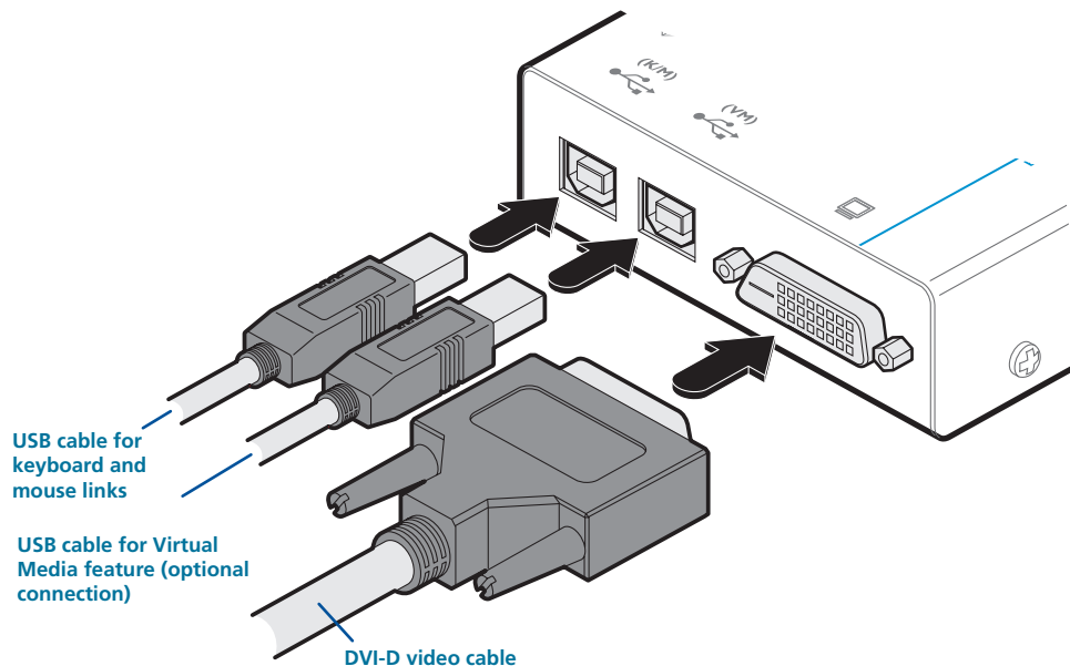
Figure 3-3. Connecting the video and USB cables
