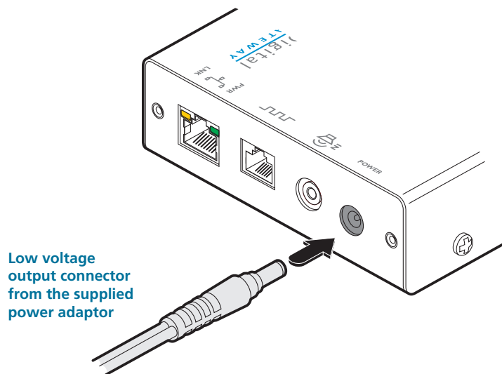
Figure 3-7. Connecting the power adaptor
