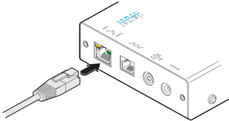
Figure 4-1. Connect to an IP network where a computer is available on the same subnet
