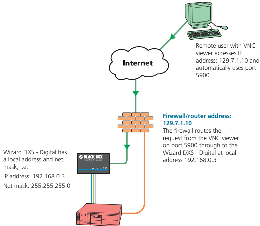
Figure E-3. Wizard DXS - Digital addressing within the network
