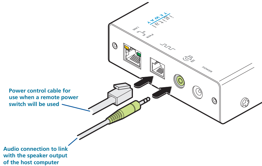
Figure 3-4. Connecting the optional audio and power control cables
