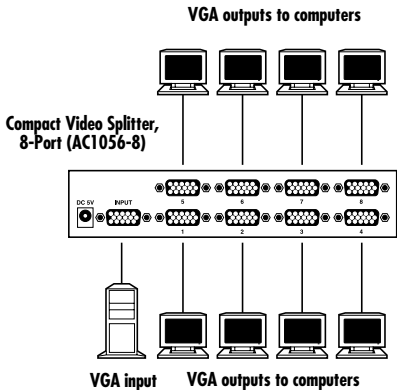
Figure 3-1. Compact Video Splitter, 8-Port (AC1056-8) connection.
